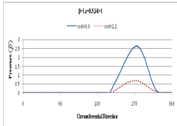
Fig:3- Pressure Distributions in Circumferential Direction
